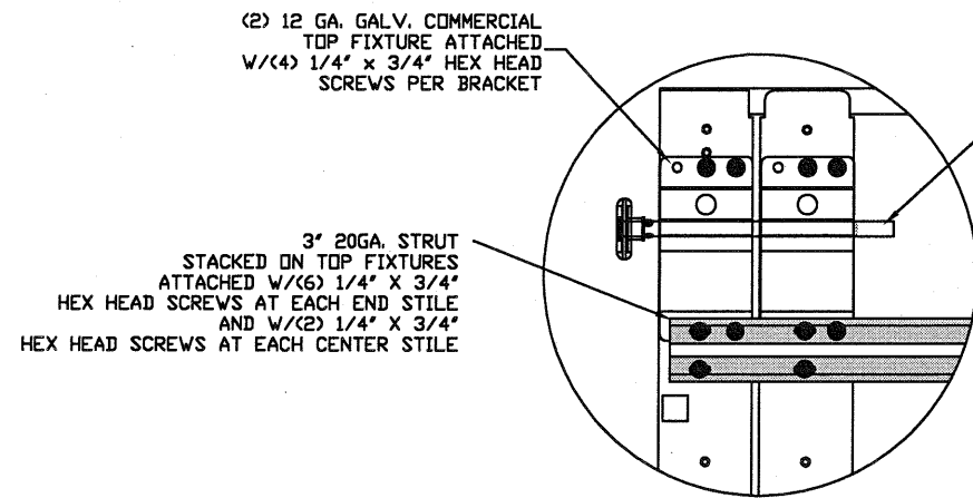
TYPICAL TOP FIXTURES N.T.S.
